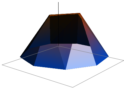
Figure: Piecewise linear ( P_1 )-approx. (conventional)
