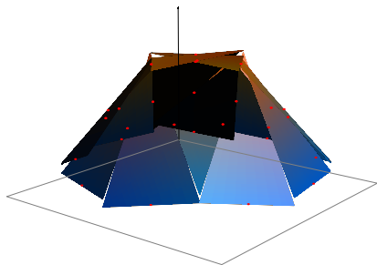
Figure: Crouzeix-Raviart element
